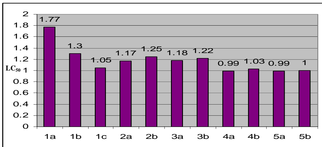
Figure 1: \text{LC}_{50} values of the synthesized compounds 1a - 5b .
