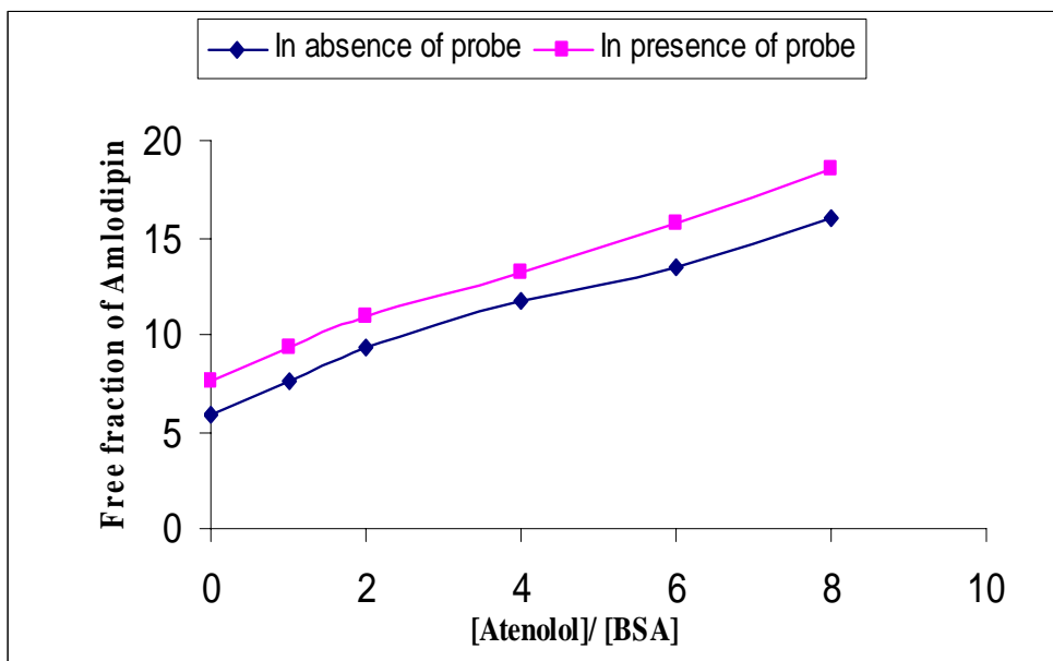
Figure 1: Displacement of amlodipine (20 \mu\text{M} ) from its binding site to BSA upon addition of increasing amount of atenolol from 0 to 100 \mu\text{M} concentration
