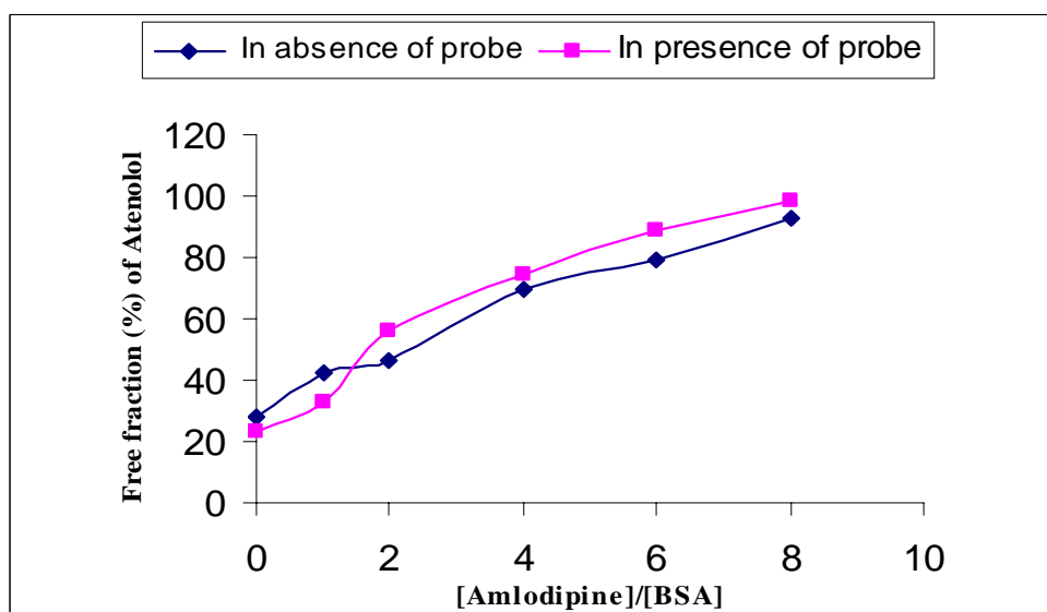
Figure 2: Displacement of atenolol (20 \mu\text{M} ) from its binding site to BSA upon addition of increasing amount of amlodipine from 0 to 100 \mu\text{M} concentration
