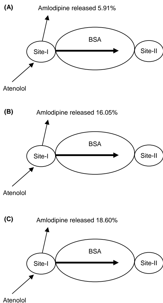
Figure 3: Proposed models of the amlodipine-BSA-atenolol interaction in presence and absence of warfarin (site-I specific probe) Concentrations were used: [BSA] = [Amlodipine] = 20 \mu M; [Atenolol] = 160 \mu M; [Warfarin] = 40 \mu M. (A) Normal condition of binding; (B) Drug interaction in absence of probe; (C) Drug interaction in presence of probe
